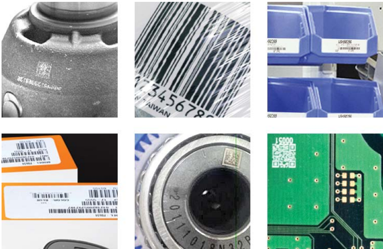
Figure 19: Barcode symbologies
