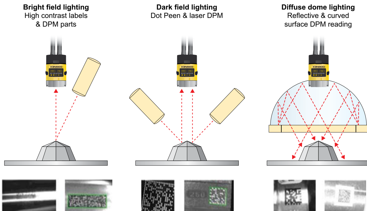
Figure 17: Lighting technology
