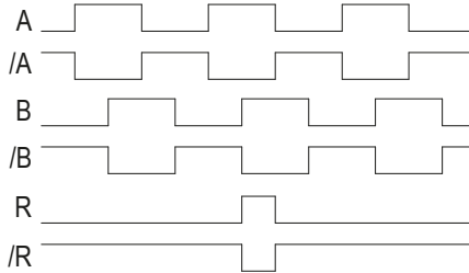
Fig. 9: Signal sequence
