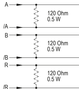
Fig. 8: Connection note
