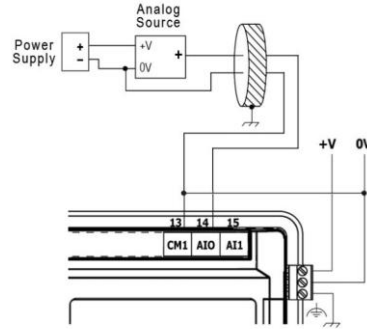
Single-ended
