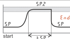
Fig 3d: Timer mode 6
