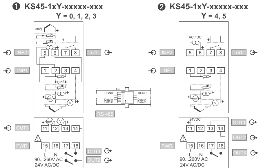
Fig. 1: Connecting diagram (1 = Version 1, 2 = Version 2)
