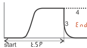
Fig 3b: Timer modes 3 and 4
