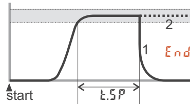
Fig 3b: Timer modes 3 and 4
