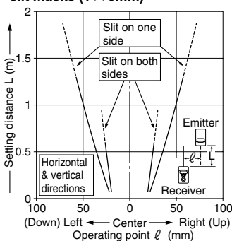
Parallel deviation with rectangular slit masks (1 × 6mm)
