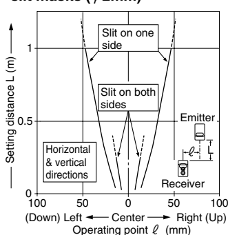
Parallel deviation with round slit masks (φ2mm)
