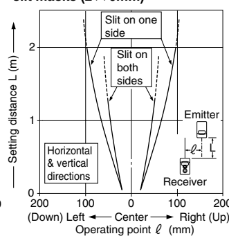
Parallel deviation with rectangular slit masks (2 × 6mm)
