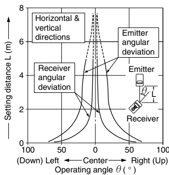
Parallel deviation with rectangular slit masks (0.5 × 6mm)
