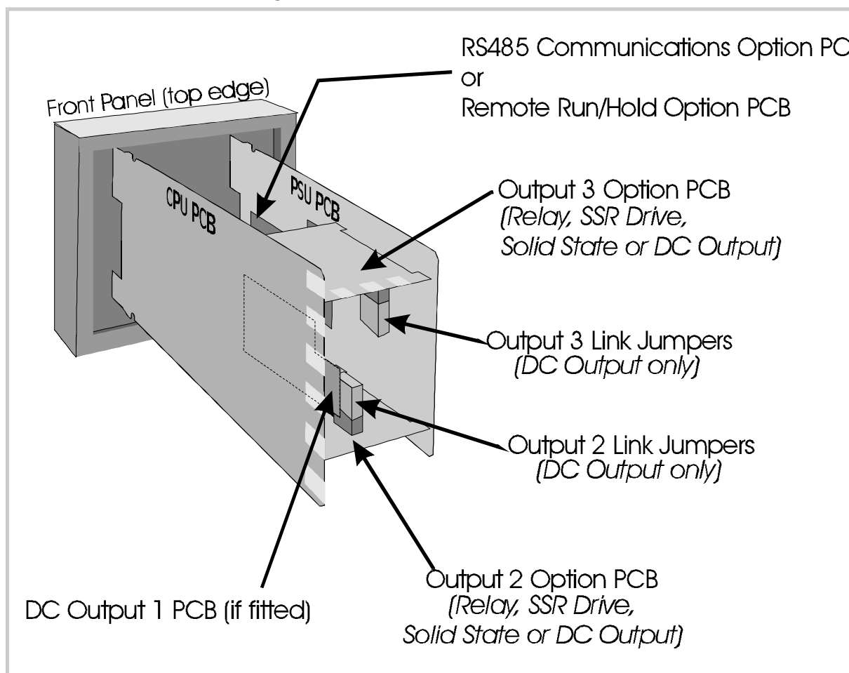
Figure 2-1 PCB Positions
