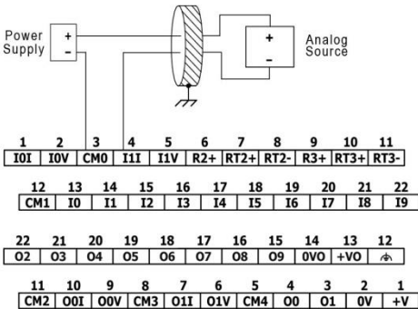
4-wire
