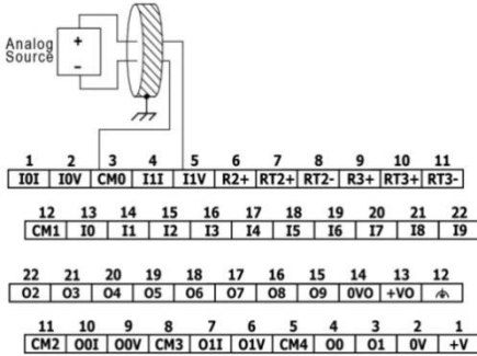
Differential
