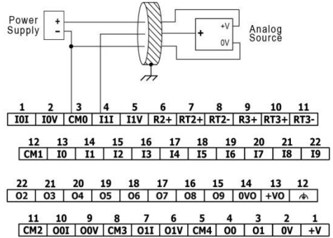
3-wire
