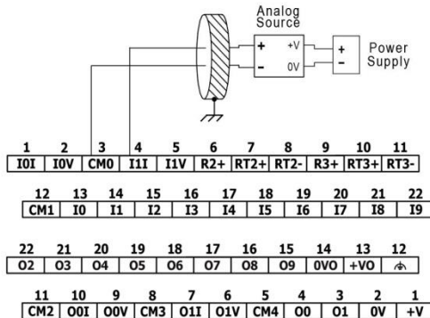
4-wire
