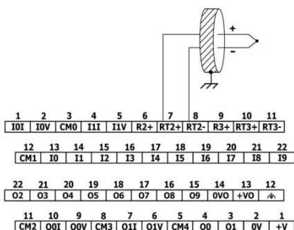
Thermocouple
