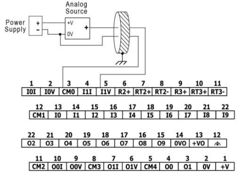
Single-ended
