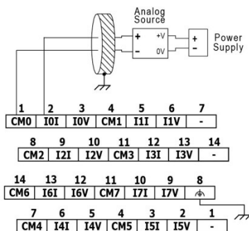
4-wire
