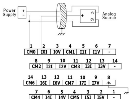
3-wire
