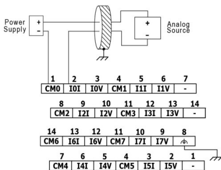
2-wire
