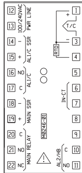
Fig. 3.A TERMINAL BLOCK (for 100/240 V AC models)
